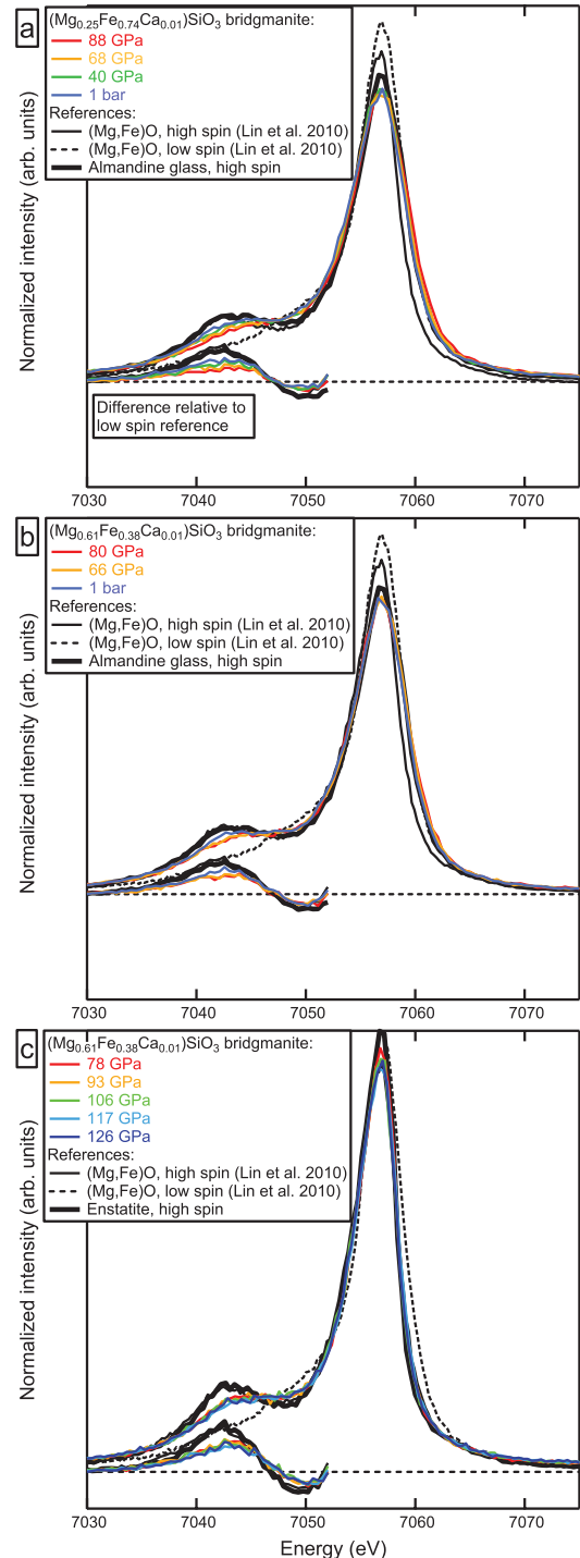
FIGURE 3. X-ray emission spectra and difference spectra relative to low-spin reference observed on decompression at APS 16-ID-D (a and b) and compression at Soleil GALAXIES (c) for (\text{Mg}_{0.25}\text{Fe}_{0.74}\text{Ca}_{0.01})\text{SiO}_3 (a) and (\text{Mg}_{0.61}\text{Fe}_{0.38}\text{Ca}_{0.01})\text{SiO}_3 (b and c) compositions (colored lines). Reference spectra for (\text{Mg}_{0.75}\text{Fe}_{0.25})\text{O} at ambient conditions (high spin, solid black line) and 90 GPa (low spin, dashed black line) (Lin et al. 2010b) and almandine-composition glass and enstatite measured at ambient conditions at HPCAT and GALAXIES, respectively, are also shown (high spin, bold black line). (Color online.)
