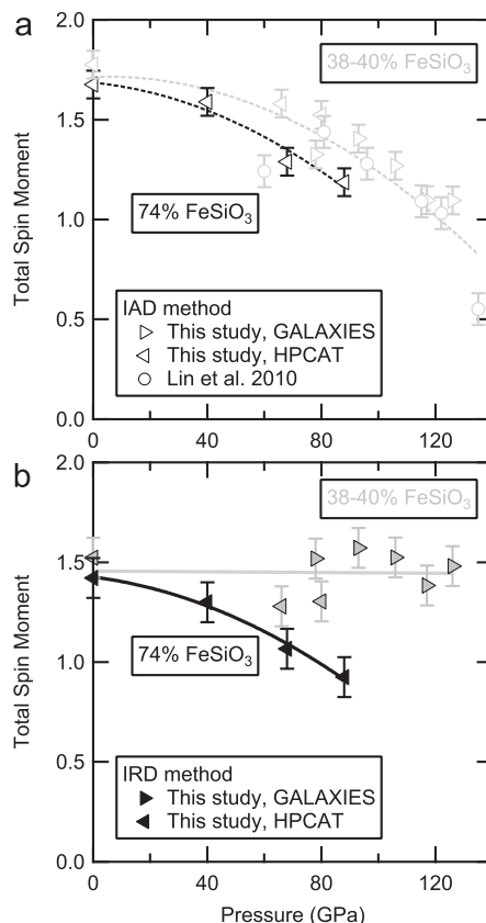
FIGURE 4. (a) Total spin moment calculated from integrated absolute difference (Vankó et al. 2006) between measured spectra and reference high- and low-spin spectra for (\text{Mg}_{0.75}\text{Fe}_{0.25})\text{O} (Lin et al. 2010b). Black triangles represent (\text{Mg}_{0.25}\text{Fe}_{0.74}\text{Ca}_{0.01})\text{SiO}_3 -composition bridgmanite while gray triangles represent (\text{Mg}_{0.61}\text{Fe}_{0.38}\text{Ca}_{0.01})\text{SiO}_3 -composition bridgmanite. Gray circles represent measurements of (\text{Mg}_{0.60}\text{Fe}_{0.40})\text{SiO}_3 -composition bridgmanite by Lin et al. (2010a). Direction of triangle points indicates compression (APS 16-ID-D) or decompression (Soleil GALAXIES). A loss of spin moment is observed above 40 GPa for 74% FeSiO 3 . (b) Total spin moment calculated from integrated relative difference method (Mao et al. 2014).
