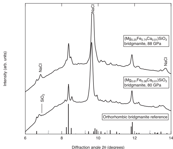
FIGURE 1. X-ray diffraction patterns of synthesized Fe-bearing bridgmanites at 300 K and reference stick pattern for orthorhombic bridgmanite. Gray starred reference sticks are additional peaks predicted by Caracas et al. (2014) for low-spin bridgmanite. X-ray wavelength is \lambda = 0.3344 for these measurements.
