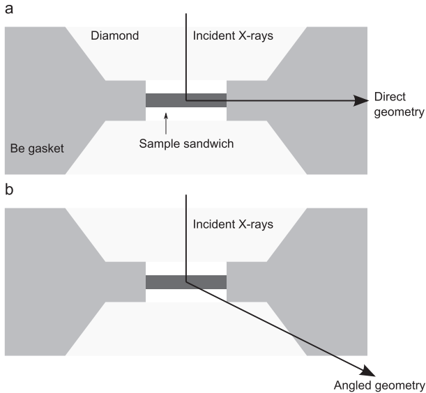
FIGURE 2. Experimental geometries for X-ray emission spectroscopy at (a) HPCAT and (b) GALAXIES beamlines.
