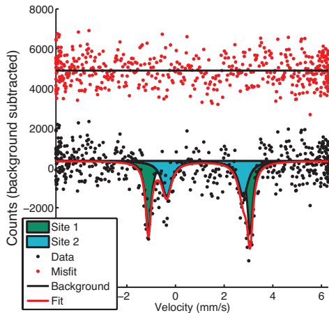
FIGURE 5. Energy-domain synchrotron Mössbauer spectrum recorded over ~18 h at beamline ID18 of the European Synchrotron Radiation Source for Fe#38-bridgmanite at 126 GPa after XES experiment. The fit is a two-site model with a Lorentzian profile (Prescher et al. 2012). Site 1 has center shift of 0.98 mm/s, quadrupole splitting of 4.18 mm/s, and intensity of 55%, and site 2 has center shift of 1.21 mm/s, quadrupole splitting of 3.15 mm/s, and intensity of 45%. Sites are identified by analogy to experiments on ^{57}\text{Fe} -enriched bridgmanite samples (Lin et al. 2008; Dorfman et al. 2014). (Color online.)
