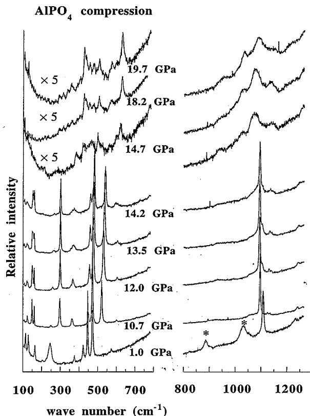
FIG. 1. High-pressure Raman spectra of \alpha -AlPO 4 taken during compression in hydrostatic pressure transmitting medium (16:4:1 methanol/ethanol/water mix). Between 14 and 15 GPa the samples undergo a polymorphic transition to a crystalline phase which is highly disordered. The spectrum contains too much structure to be amorphous, and the crystalline peaks become better defined as the pressure is increased. The peaks labeled by stars are due to the pressure-transmitting medium.
