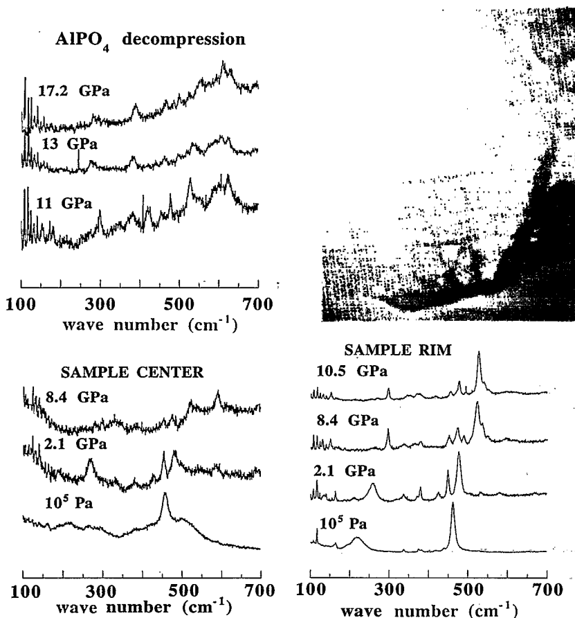
FIG. 4. Raman spectra recorded during sample decompression in quasihydrostatic (KBr) runs. From 18 to 10.5 GPa Raman spectra are identical throughout the sample. The back transformation of the sample begins below 10.5 GPa, with the reappearance of peaks of the \alpha -AlPO 4 spectrum. At this point, the rim of the sample develops a different birefringence from the interior of the grain. Systematic differences in the Raman spectra are observed on the same grain between the rim and the interior. On recovery, the grain center is isotropic, and exhibits a broad band Raman spectrum due to amorphous AlPO 4 . The superimposed sharper peaks are due to \alpha -AlPO 4 either coexisting with the glassy material in the interior of the grain, or in the surrounding rim. The \alpha -AlPO 4 peaks are shifted and broadened compared with their starting values (see details in Fig. 5). The photomicrograph shows a sample recovered after compression in KBr to 27 GPa but similar features are observed in samples compressed to 18 GPa and subsequently decompressed. The sample is examined in crossed polars with a gypsum plate. Note also the cracks developed from the edge of the sample, indicating the release of tensile stresses developed within the sample. The grain size is 120 \mu m.
