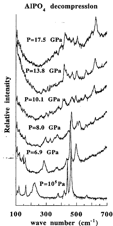
FIG. 3. Raman spectra of \text{AlPO}_4 taken during decompression in hydrostatic pressure media (ethanol:methanol:water mix). The backtransformation from the high-pressure phase to \alpha - \text{AlPO}_4 occurs below 8 GPa. The room-pressure spectrum is similar but weaker than that of the starting material.
