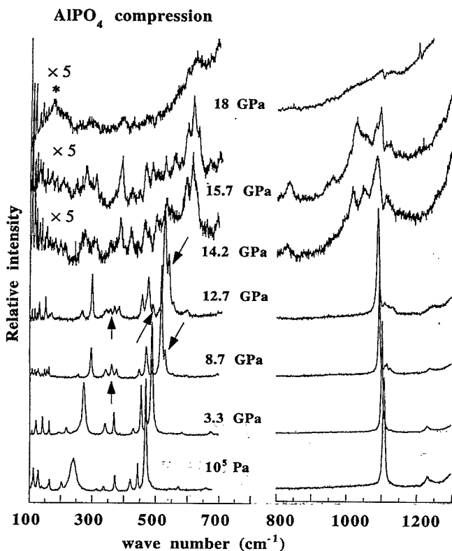
FIG. 2. High-pressure Raman spectra of \alpha - \text{AlPO}_4 taken during compression in KBr. Note the splitting of some modes (arrows) due to shear stresses developed in the sample because of the quasihydrostatic nature of the pressure-transmitting medium. Above 13 GPa the sample undergoes a polymorphic transition similar to that observed in the hydrostatic runs. The spectra of the high-pressure phases obtained in the hydrostatic and quasihydrostatic experiments are similar, but not identical. Above 18 GPa in the quasihydrostatic experiment, the broad Raman bands indicate the sample may be amorphous. Bands labeled by stars are second-order features of KBr.
