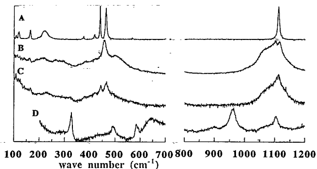
FIG. 6. Raman spectra of AlPO 4 recovered from compression experiments of \alpha -AlPO 4 using different pressure-transmitting media: (A) compressed to 20 GPa in 16:4:1 methanol/ethanol/water mix. (B) compressed to 18 GPa in KBr. Note the broad bands due to the recovered amorphous phase. (C) compressed to 27 GPa in KBr. (D) compressed to 25 GPa without pressure-transmitting medium. Note the additional sharp peaks in the spectrum, due to appearance of a crystal phase on decompression. These could be due to a rutile-like phase, or to a phase with the InPO 4 ( Cmcm ) structure.
