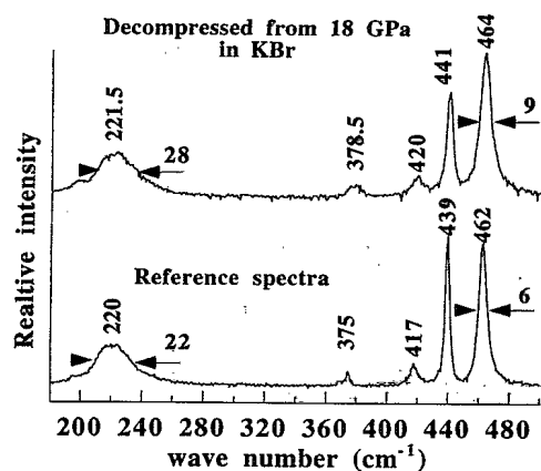
FIG. 5. Raman spectrum of \alpha -AlPO 4 after decompression from 18 GPa and KBr (sample rim, see Fig. 4) compared to the Raman spectrum of an uncompressed sample. The peak wavenumbers as well as the bands full width at half maximum are indicated.
