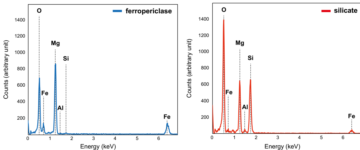
Fig. S2. EDX spectra for (Left) Fp and (Right) silicate. Energy distribution corresponds to X-ray emissions from characteristic chemical elements. Peak height is correlated to element concentration in the investigated zone. The spectrum for Fp shows no peak for Si and Al, in good agreement with the absence of these two elements in the mineral structure.
